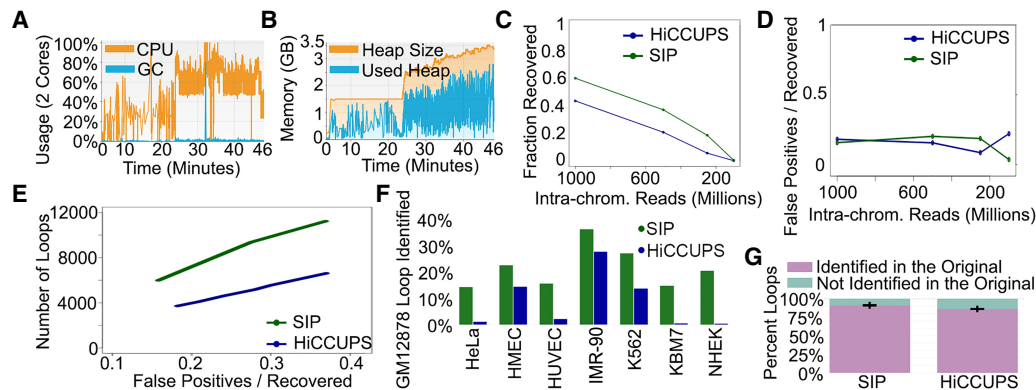
Figure 2. Performance of SIP. (A) CPU usage (orange) and GC (garbage collection, blue) over time using two cores during SIP loop calling. (B) Memory usage of SIP during loop calling. (C) Fraction of loops called using the full data set recovered by SIP (green) or by HiCCUPS (blue) in data down-sampled to different sequencing depths. (D) Ratio of false positives (loops not identified in the full data set) versus loops recovered by SIP (green) or HiCCUPS (blue) in down-sampled data. (E) Number of loops identified in down-sampled data ( y -axis) for SIP (green) and HiCCUPS (blue) when parameters were adjusted to give the same false positive/recovery rate ( x -axis). (F) Percentage of loops identified by SIP (green) or HiCCUPS (blue) in GM12878 cells that were identified in a different cell type. (G) Percentage of loops identified in each permutation down-sampling data (purple) versus new loops (i.e., false positives) (teal). Bars represent averages of 10 permutations with error bars representing standard deviation.
